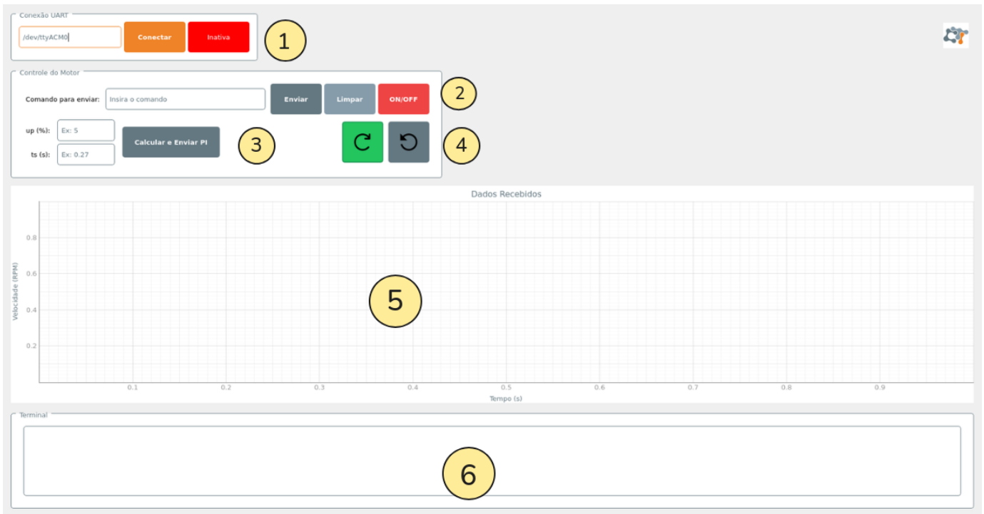
Fig. 12: Graphical interface
