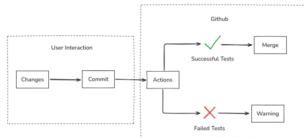
Fig. 13: Github Actions Workflow Diagram
