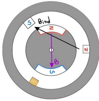
(a) Magnetic Fields at the BLDC
