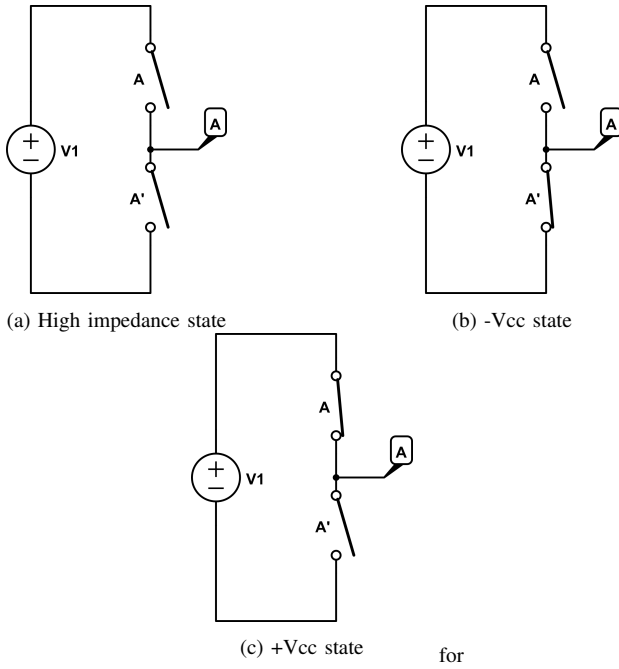
Fig. 6: Illustration of different phase states for motor control
